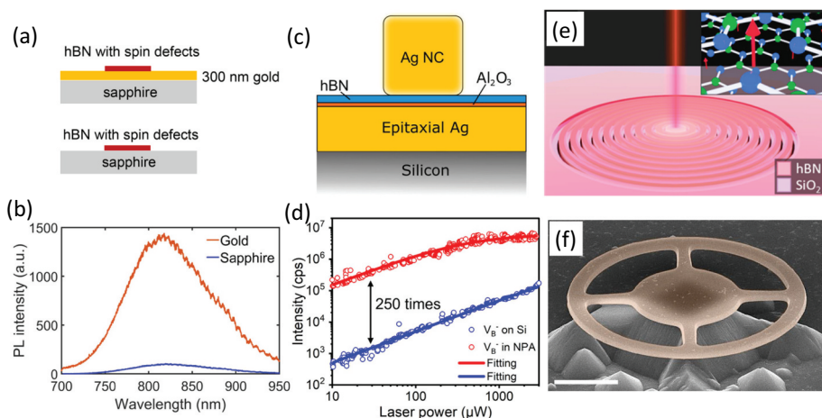
Figure 12. (a) Schematic of an hBN flake deposited on a gold-coated sapphire substrate or on a bare sapphire substrate. (b) Increased photoluminescence intensity from hBN V_B^- defects deposited on a gold-coated sapphire substrate. Reproduced from [28]. Copyright by American chemical society. (c) Schematic of a plasmonic nanocavity formed between a silver nanocube and an epitaxial silver film separated by ultrathin hBN and Al 2 O 3 thin films. (d) Increased photoluminescence intensity as a function of laser power for hBN spin defects in a silver nanocavity. Reproduced from [130]. Copyright by American chemical society. (e) Schematic of a bullseye cavity fabricated out of hBN with the emission being coupled out of plane for maximum collection. Reproduced from [131]. Copyright by American chemical society. (f) SEM image of a hBN/TiO 2 ring resonator fabricated to increase emission. Reproduced from [132]. Copyright by royal society of chemistry. Scale bar: 2 μm.
